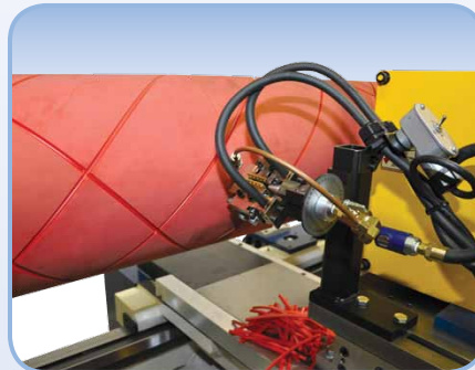
Thermocutter (Hot Knife) Grooving Option
