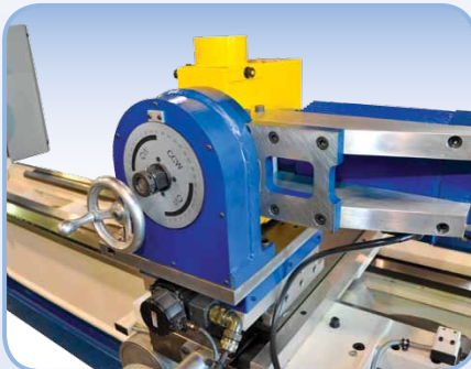
Custom-Made Tilting Groover/Grinder
