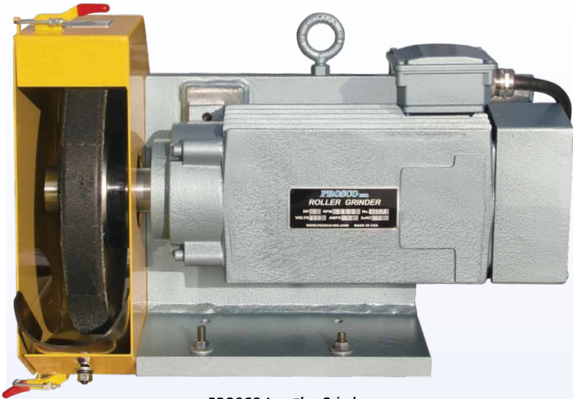
PROSCO Inc. 5hp Grinder with 12 inch wheel
